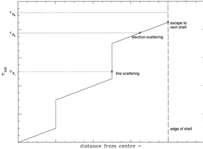
Fig. 3.3 The process of choosing a scattering location in a cell. Credit Mazzali and Lucy 1993
