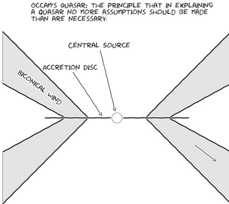
Fig. 1.15 Occam's quasar. How far can this general picture take us when trying to explain the behaviour of quasars and other accreting compact objects?
