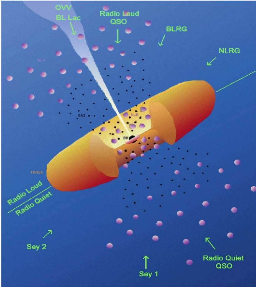
Fig. 1.13 A unified scheme for AGN. The broad line region is compact and can thus be obscured from view by a dusty torus, whereas the larger narrow line region is always visible. The radio-loud/radio-quiet dichotomy is explained by the presence or absence of a radio jet. Credit Modified from Urry and Padovani (1995). Copyright PASP, reprinted by permission of the authors
