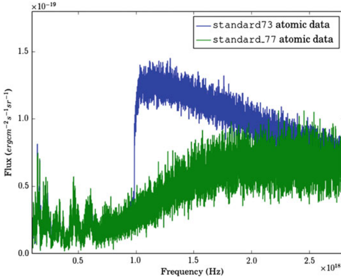
Fig. 3.8 A comparison of the soft X-ray regime of the H13 model, with two different datasets. standard73 is the dataset with old, unextrapolated cross-sections and standard77 instead includes extrapolated cross-sections as described in the text
