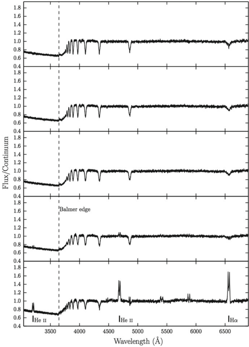
Fig. 4.5 Synthetic optical spectra from model A computed for sightlines of 10, 27.5, 45, 62.5 and 80°. In these plots the flux is divided by a polynomial fit to the underlying continuum redward of the Balmer edge, so that line-to-continuum ratios and the true depth of the Balmer jump can be shown
