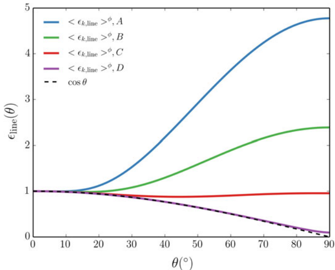
Fig. 6.15 The azimuthally-averaged line angular emissivity function, \bar{\epsilon}_{k,\text{line}} , from a Keplerian disc as a function of inclination angle for the four models shown in Table 6.1. The model parameters are the values of H/R , v_k and v_{th} . The zero Keplerian velocity shear case, \epsilon_{0,\text{line}}(\theta) = \cos \theta (dotted line), is also shown. Unless the disc is very thin ( H/R \sim 0.001 ), \bar{\epsilon}_{k,\text{line}} shows large deviations from \cos \theta
