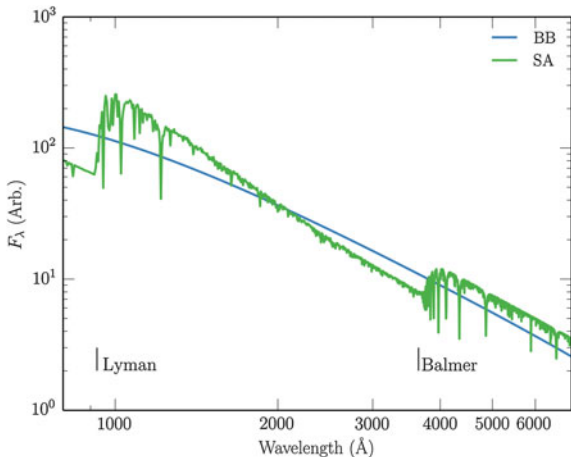
Fig. 1.5 A comparison between a disc spectrum computed with stellar atmosphere models and standard multi-temperature blackbody disc. The major photoabsorption edges are marked. Flux is reprocessed into different wavelengths by bound-free opacities, and line blanketing also has a big effect on the spectrum. The Hydrogen and Helium lines also experience a degree of pressure broadening
