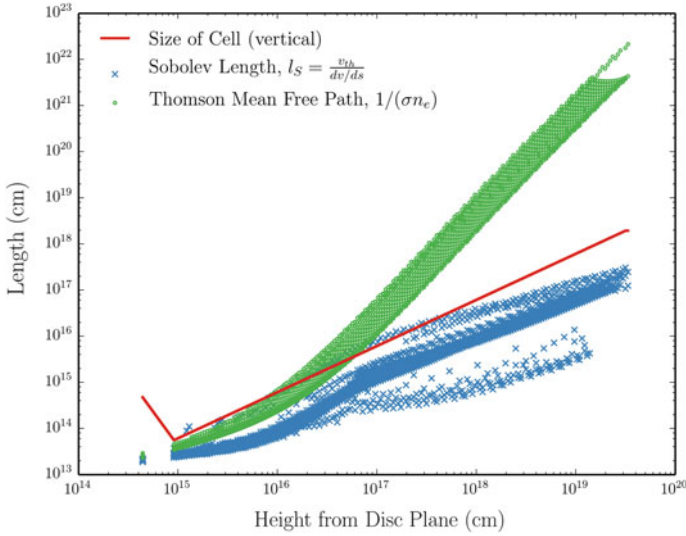
Fig. 5.3 Some typical length scales for the fiducial model. This places a formal limit of \sim 10^{12} cm on clump sizes in the microclumping framework, and confirms that the cells are sufficiently larger than the Sobolev length in almost all cases
