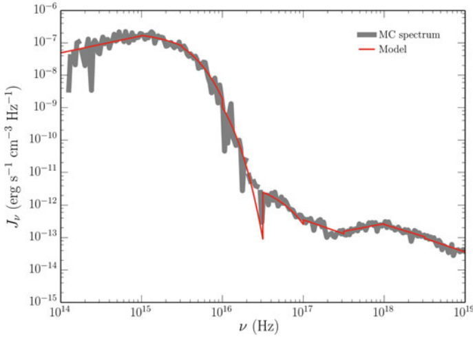
Fig. 3.5 An example of a modeled spectrum in PYTHON compared to the recorded MC spectrum, from an individual cell in an AGN model
