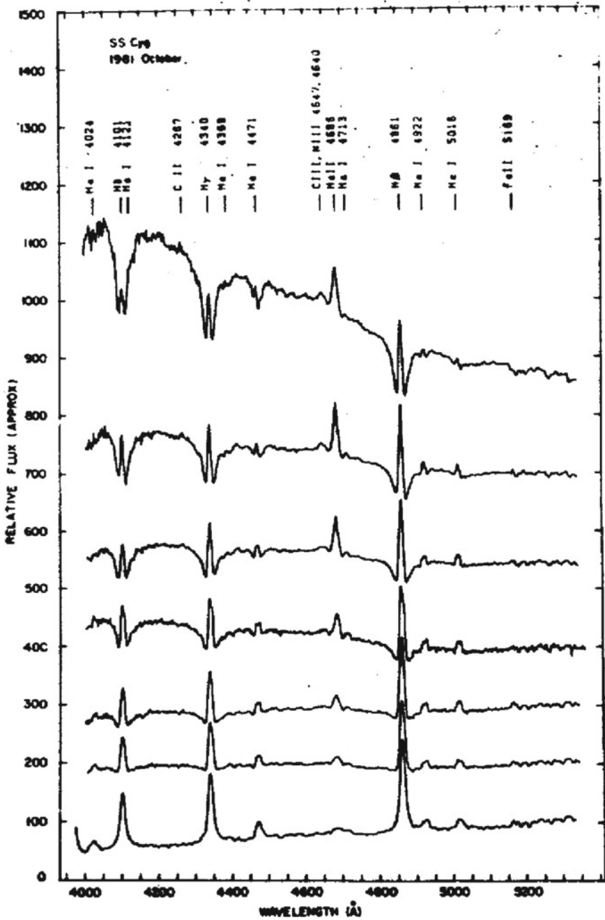
Fig. 1.9 Spectra of SS Cyg during an outburst cycle, showing the evolution from minimum to maximum light. The rise is characterised by the appearance of an optically thick accretion disc spectrum. The flux scale is approximate. Credit Hessman et al. 1984/Dhillon 1996
