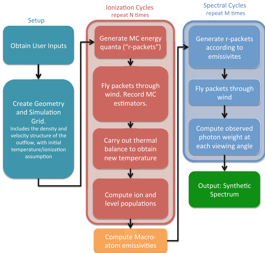
Fig. 3.2 A flowchart showing the basic operation of PYTHON
