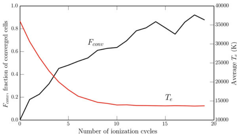
Fig. 3.6 The average temperature and fraction of converged cells in a typical CV model, shown as a function of the number of ionization cycles completed
