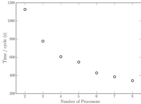
Fig. 3.19 Total runtime per cycle for an AGN run as a function of the number of processors
