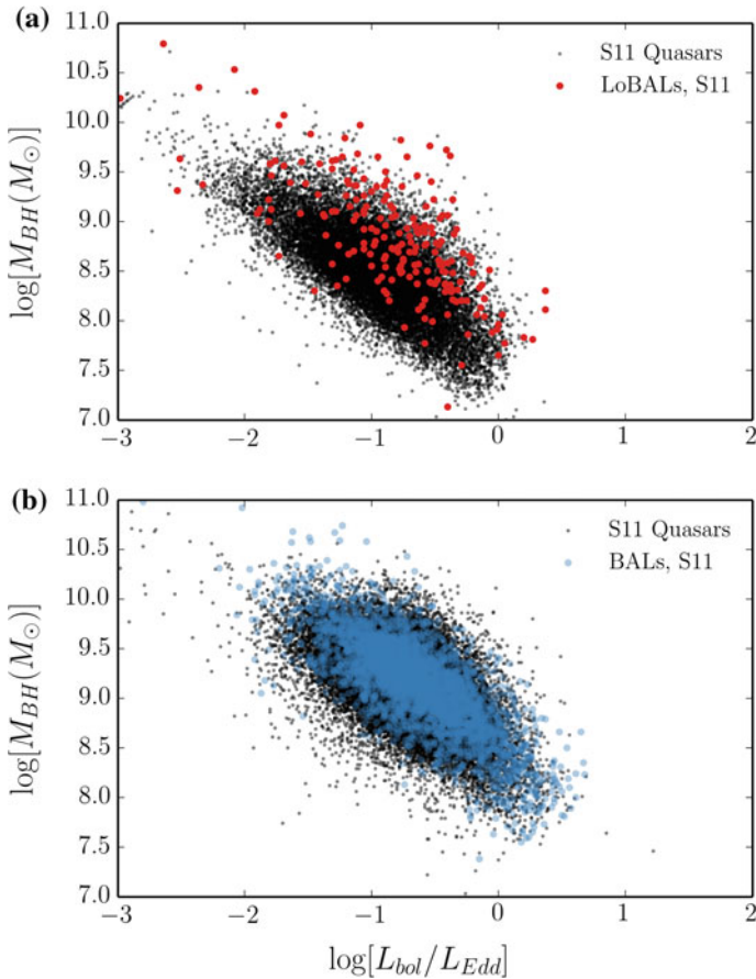
Fig. 6.1 BH mass and Eddington fraction measurements from S11 for Sample A ( top ) and Sample B ( bottom ). The LoBALQSOs in sample A and BALQSOs in Sample B are also plotted in each case
