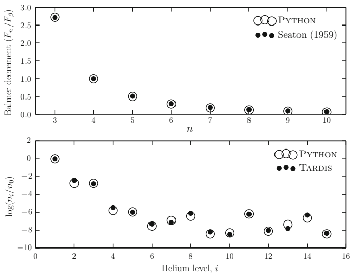
Fig. 3.15 Top Panel ‘Case B’ Balmer decrements computed with PYTHON compared to analytic calculations by Seaton (1959). Both calculations are calculated at T_e = 10,000\text{K} . Bottom Panel a comparison of He I level populations (the most complex ion we currently treat as a macro-atom) between PYTHON and TARDIS models. The calculation is conducted in thin shell mode with physical parameters of n_e = 5.96 \times 10^4 \text{ cm}^{-3} , T_e = 30,600\text{K} , T_R = 43,482\text{K} and W = 9.65 \times 10^{-5}
