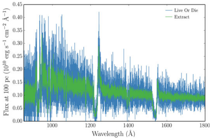
Fig. 3.7 A synthetic spectrum after 30 spectral cycles with 100, 000 photons from simple CV wind model at a 60^\circ viewing angle. Spectra produced with both the extract and live or die modes are shown. The effectiveness of the extract variance reduction technique can be clearly seen, and we can see that the spectral shape is unaltered
