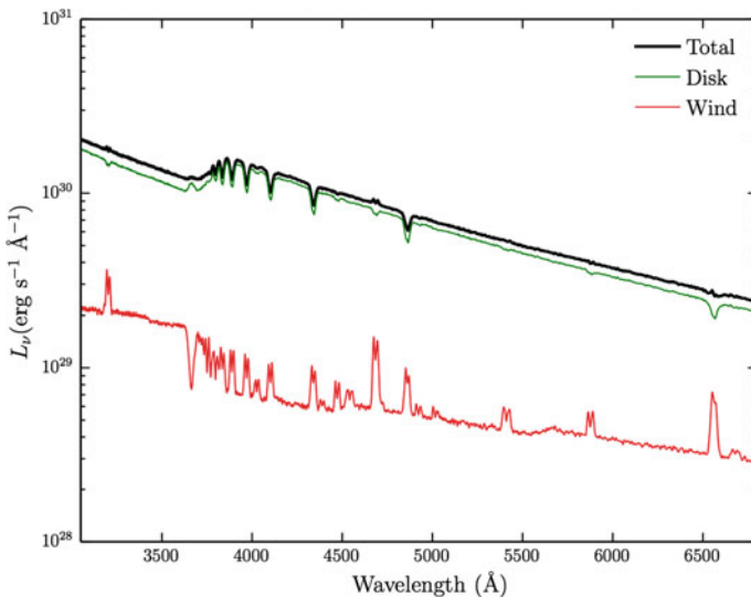
Fig. 4.6 Total packet-binned spectra across all viewing angles, in units of monochromatic luminosity. The thick black line shows the total integrated escaping spectrum, while the green line shows disc photons which escape without being reprocessed by the wind. The red line show the contributions from reprocessed photons. Recombination continuum emission blueward of the Balmer edge is already prominent relative to other wind continuum processes, but is not sufficient to fill in the Balmer jump in this specific model
