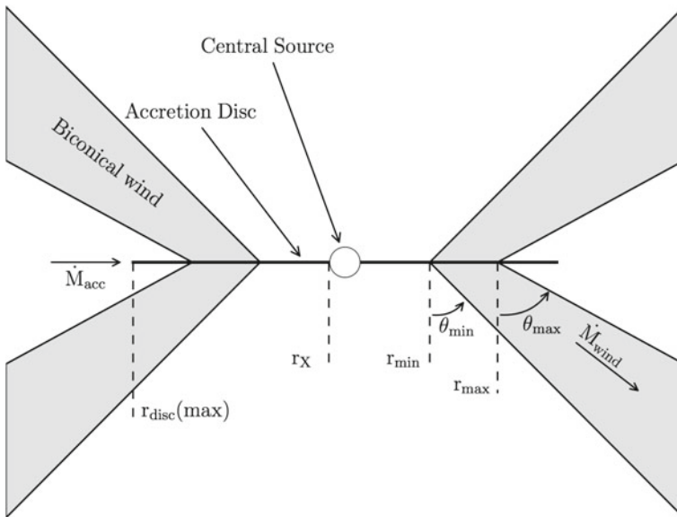
Fig. 5.1 A cartoon showing the geometry and some key parameters of the biconical quasar wind model
