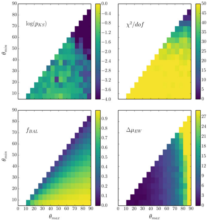
Fig. 6.8 Heat map showing the results of the MC simulation described in Sect. 6.4.2. The quantities shown are discussed further in the text, but correspond to (clockwise from top left ): the p_{KS} value from a comparison between the mock BAL dataset and the observed BAL dataset, the reduced \chi^2 from the fit to the non-BAL EW distribution, the difference in mean EW between the mock BAL and mock non-BAL datasets, and the BAL fraction expected for the geometry in question
