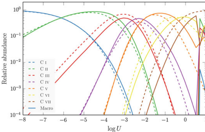
Fig. 7.1 Ion fractions as a function of ionization parameter when Carbon is treated as a simple-atom (dotted lines) or macro-atom (solid lines) Although serious, as yet unsolved, numerical problems appear at high ionization parameters, the fundamental machinery for treating Carbon as a macro-atom is now in place
