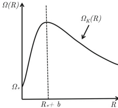
Fig. 1.2 Angular velocity as a function of radius in an accretion disc around a rotating compact object with angular velocity \Omega_* . \Omega_K is the Keplerian angular velocity. This graph also helps explain why there is a turnover in the temperature–radius relation, as D(R) is proportional to the square of the derivative of this quantity. The boundary condition responsible for this turnover is briefly discussed in the text
