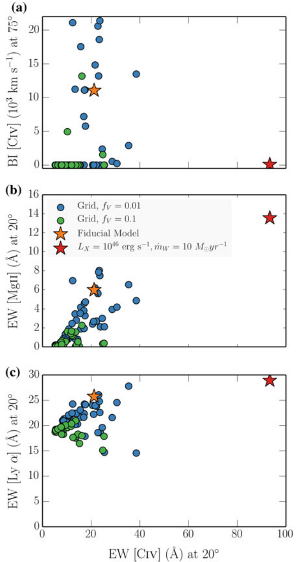
Fig. 5.11 The EW of the C IV 1550 Å line at 20° plotted against a the BI of C IV 1550 Å at 75°, b the EW of the Mg II 2800 Å line at 20° and c the EW of Ly \alpha at 20°. The circles correspond to the simulation grid for two different values of f_V , and the fiducial model is marked with an orange star. I also show a higher X-ray luminosity model and a higher mass loss rate with a red star
