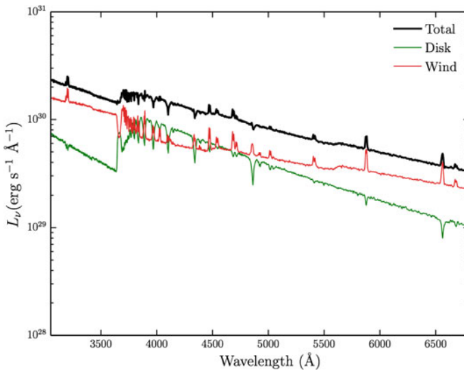
Fig. 4.9 Total packet-binned spectra across all viewing angles, in units of monochromatic luminosity. The thick black line shows the total integrated escaping spectrum, while the green line shows disc photons which escape without being reprocessed by the wind. The red line show the contributions from reprocessed photons. In this denser model the reprocessed contribution is significant compared to the escaping disc spectrum. The Balmer continuum emission is prominent, and the wind has a clear effect on the overall spectral shape
