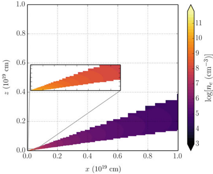
Fig. 5.5 The electron density in the model, this time on linear axes in order to illustrate the density contrasts and scale of the system. The plot is on the scale of the acceleration length, whereas the inset is a box of 2700 \times 800 r_G , where the bottom left corner corresponds to the base of the innermost streamline
