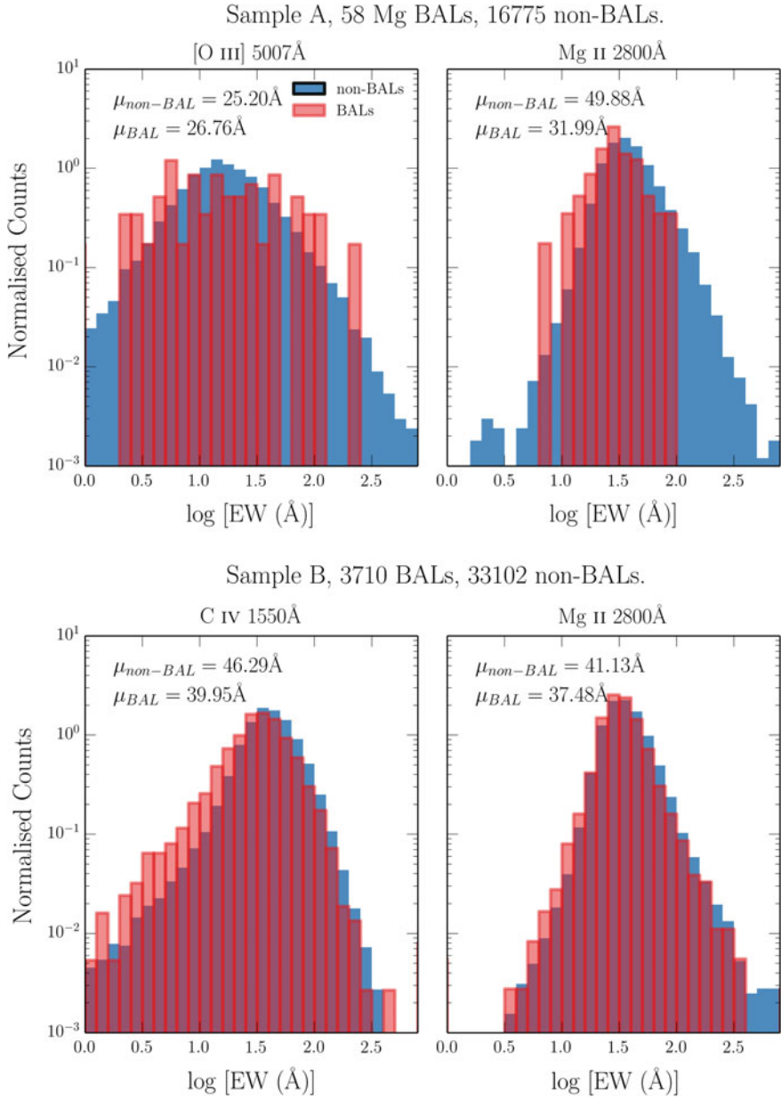
Fig. 6.2 Histograms of equivalent widths for three emission lines from the two different samples. The mean of the BAL and non-BAL quasar distributions are labeled in each case, and the histograms are normalised
