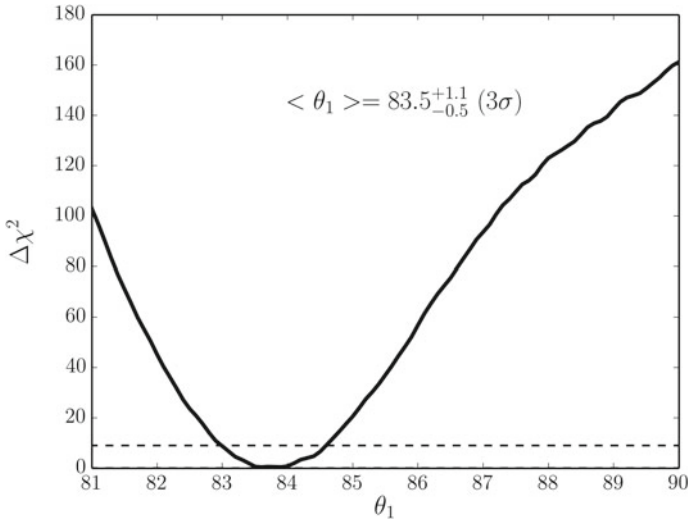
Fig. 6.6 \Delta\chi^2 as a function of maximum angle, \theta_1 , calculated in steps of 0.1^\circ . The choice for \mu_* and \sigma_* is left free in each case. The dotted line marks the 3\sigma confidence interval
