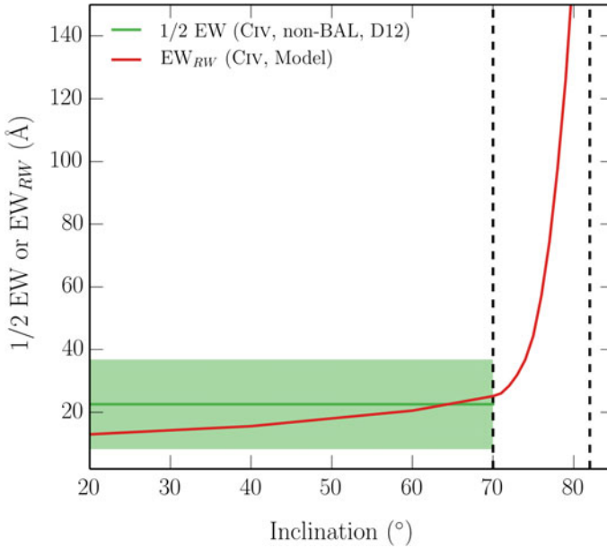
Fig. 5.12 EW_{RW} as a function of inclination in the fiducial model, compared to 1/2 EW from the quasar sample of Di Pompeo et al. (2012; D12). The shaded region corresponds to the standard deviation of the D12 sample
