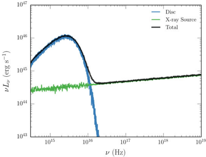
Fig. 5.2 The input spectrum used for the quasar modelling. Note that although the X-ray power law is allowed to extend to very high frequencies, the radiation beyond \sim 10^{18} Hz is unimportant due to the rapid decline in the photoionization cross-sections at high energies. The results here are thus insensitive to the maximum frequency adopted for this power law component
