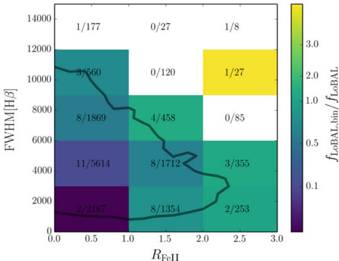
Fig. 6.11 LoBAL fraction compared to global LoBAL fraction in Eigenvector 1 space, in bins of \Delta R_{\text{FeII}} = 1 and \Delta \text{FWHM}[\text{H}\beta] = 3000 \text{ km s}^{-1} . The contour shows the outermost contour from Fig. 6.10 for reference. The text shows N_{\text{LoBAL}}/N_{\text{non-BAL}} , where N_{\text{LoBAL}} is the number of LoBAL QSOs in the bin and N_{\text{non-BAL}} is the number of non-BAL quasars in the bin
