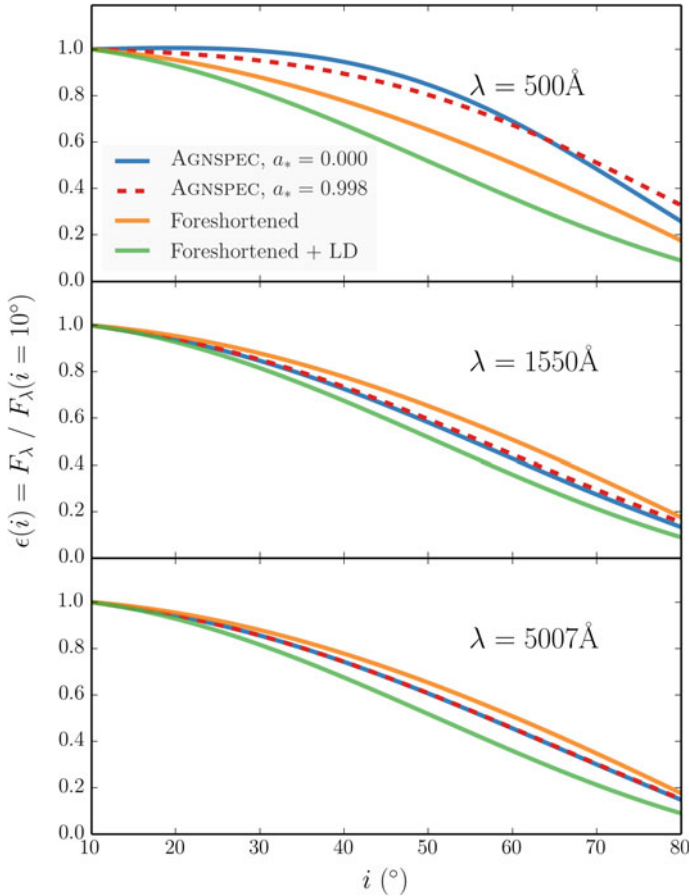
Fig. 6.3 Angular variation of continuum luminosity from AGNSPEC and classical thin disc models. The monochromatic continuum luminosities is divided by the monochromatic continuum luminosity at 10^\circ , from AGNSPEC and classical thin disc models, at three different wavelengths. The models are computed for an Eddington fraction of 0.2 and M_{BH} = 10^9 M_\odot . In each panel I show both Kerr and Schwarzschild AGNSPEC models, and the classical models are for both pure foreshortened discs and foreshortened and limb darkened (LD) discs
