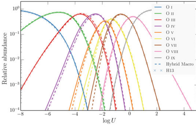
Fig. 3.13 As Fig. 3.9, but for oxygen
