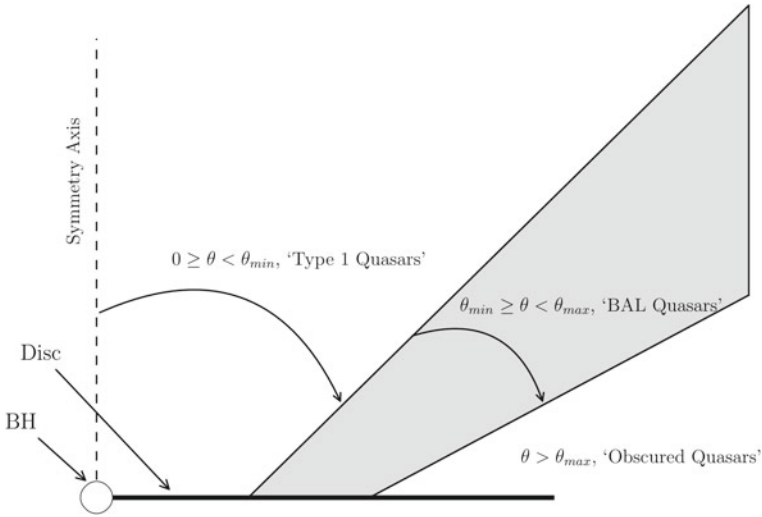
Fig. 6.7 The geometry of the toy model used to carry out the Monte Carlo simulations
