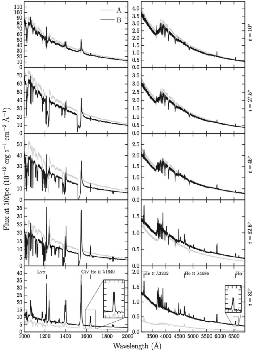
Fig. 4.7 UV ( left ) and optical ( right ) synthetic spectra for model B computed at sightlines of 10, 27.5, 45, 62.5 and 80°. Model A is shown in grey for comparison. The inset plots show zoomed-in line profiles for He II 1640 Å and H \alpha . The Balmer and He are double-peaked, albeit with narrower profiles. Strong He II 4686 Å emission can be seen, as well as a trend of a deeper Balmer jump with decreasing inclination
