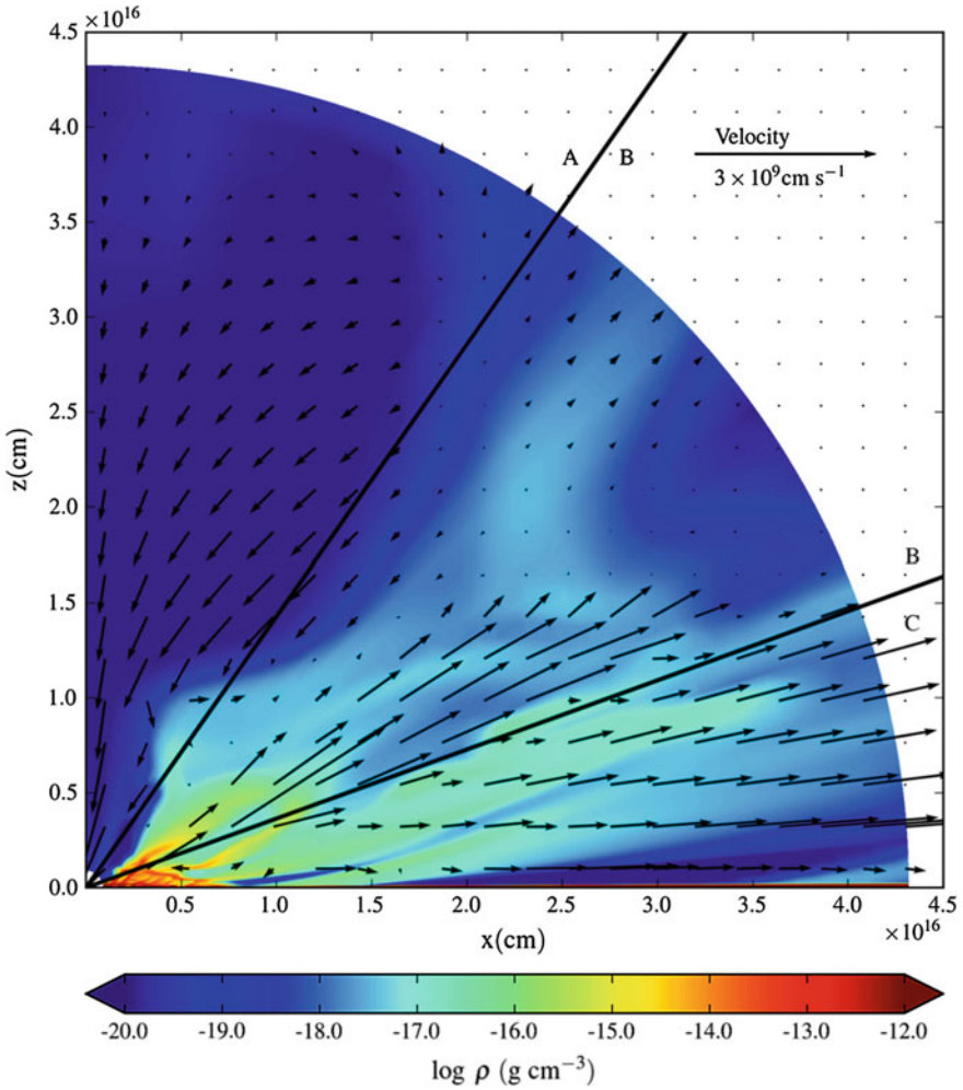
Fig. 2.13 A snapshot of the PK04 model. Colours shows the density and arrows show the velocity of the flow. The radial lines separate three areas described by H14. Credit Higginbottom et al. (2014). Copyright AAS. Reproduced with permission
