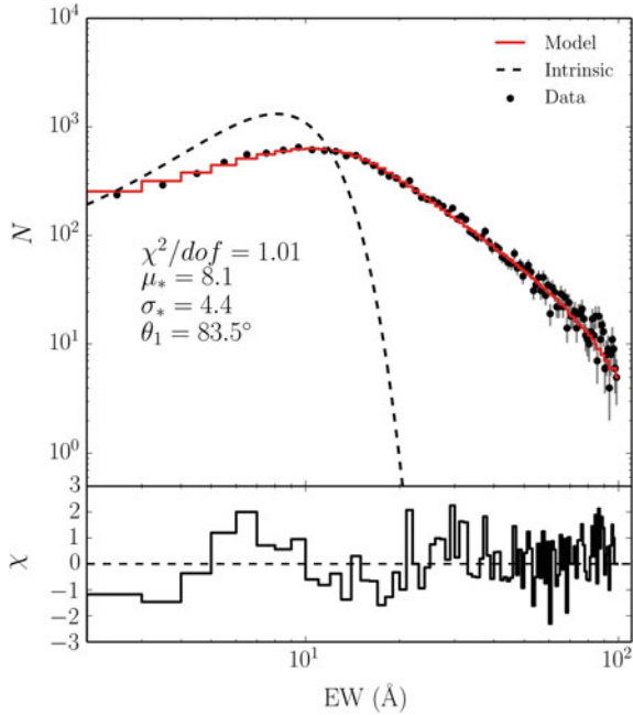
Fig. 6.5 The EW[O III] distribution of quasars in the R11 sample ( black points ), with \sqrt{N} errorbars, and the best fit model with a maximum viewing angle of 84^\circ . The intrinsic Gaussian distribution is shown with a dashed line . The plotted data is equivalent to the non-BAL histogram in the top left panel of Fig. 6.2, except that it uses linear binning and adopts the R11 sample criteria rather than using sample A
