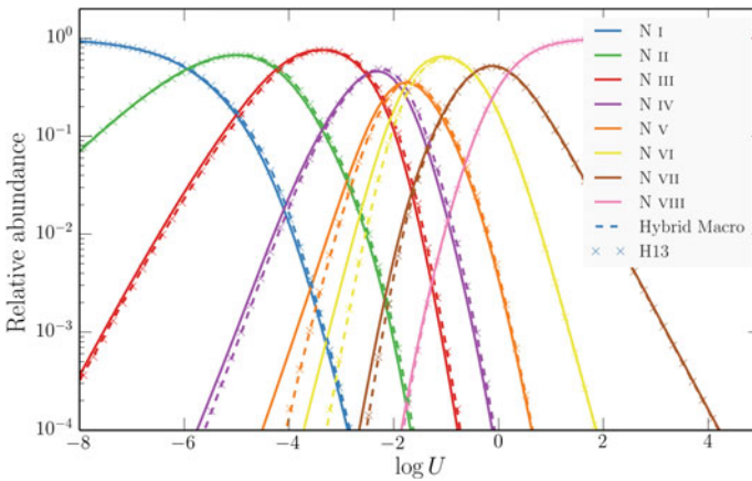
Fig. 3.12 As Fig. 3.9, but for nitrogen
