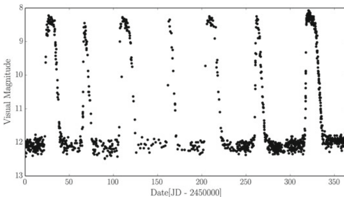
Fig. 1.8 Data AAVSO. A year in the life of SS Cyg, showing the characteristic repeated outbursts and periods of quiescence typical of a DN. SS Cyg has been undergoing this activity since it was first observed in 1896
