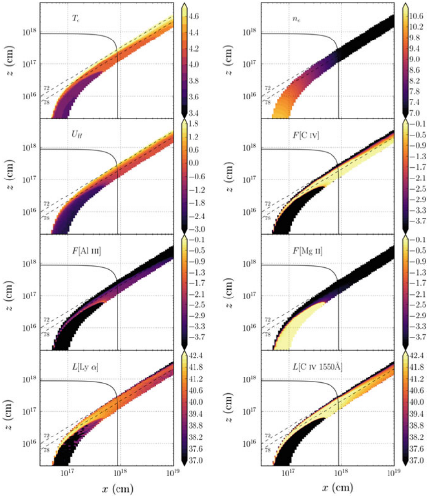
Fig. 5.4 Contour plots showing the logarithm of some important physical properties of the outflow. The spatial scales are logarithmic and the x and z scales are not the same. The panels show the electron temperature, T_e , electron density, n_e , the ionization parameter, U_H , ion fractions, F , for three different ions and line luminosities, L , for two different lines. The line luminosities represent the luminosity of photons escaping the Sobolev region for each line. These photons do not necessarily escape to infinity. The solid black line marks a sphere at 1000 r_G . The dotted lines show the 72^\circ and 78^\circ sightlines to the centre of the system, and illustrate that different sightlines intersect material of different ionization states
