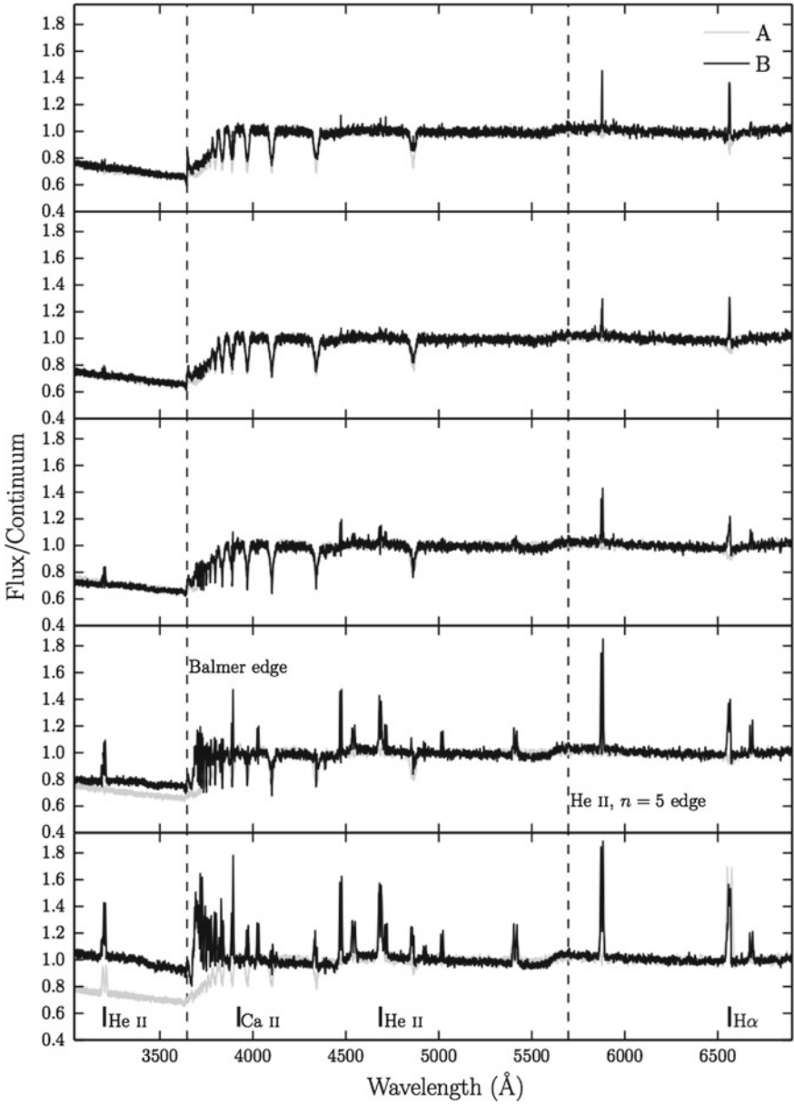
Fig. 4.8 Synthetic optical spectra from model B computed for sightlines of 10, 27.5, 45, 62.5 and 80°. Model A is shown in grey for comparison. In these plots the flux is divided by a polynomial fit to the underlying continuum redward of the Balmer edge, so that line-to-continuum ratios and the true depth of the Balmer jump can be shown
