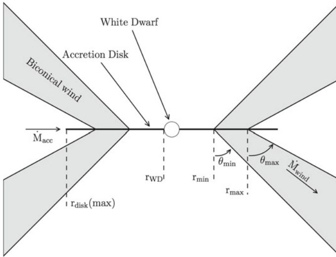
Fig. 4.1 Cartoon illustrating the geometry and kinematics of the benchmark CV wind model
