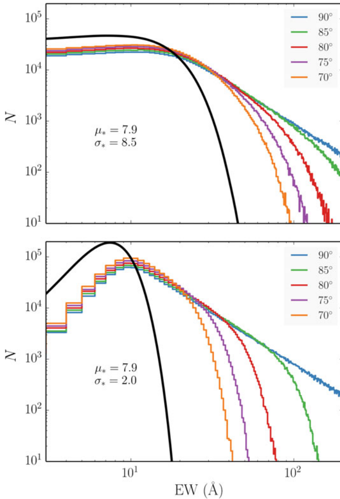
Fig. 6.4 Theoretical EW distributions from the numerical experiment described in Sect. 6.4.1 for a few different maximum angles. The results in the top panel use the same intrinsic distribution as Model 1 from R11 (shown in black ), whereas the bottom panel shows the distributions obtained from a narrower intrinsic Gaussian. By the time the maximum angle is limited to around 70^\circ the cutoff is clear even at moderate values of EW
