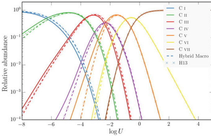
Fig. 3.11 As Fig. 3.9, but for carbon
