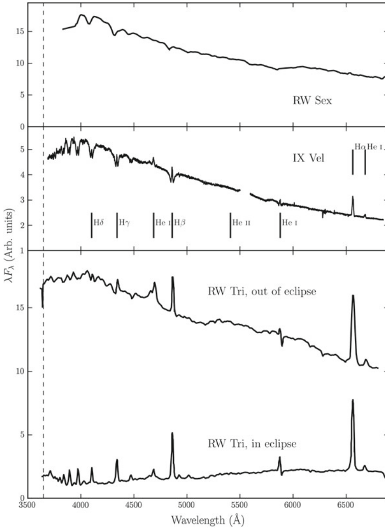
Fig. 1.11 Optical spectra of three nova-like variables: RW Sex ( top ; Beuermann et al. 1992), IX Vel ( top middle A.F. Pala and B.T. Gaensicke, private communication) and RW Tri in and out of eclipse ( bottom two panels Groot et al. 2004). The data for RW Sex and RW Tri were digitized from the respective publications, and the IX Vel spectrum was obtained using the XSHOOTER spectrograph on the Very Large Telescope on 2014 October 10. These systems have approximate inclinations of 30°, 60° and 80° respectively. The trend of increasing Balmer line emission with inclination can be seen. In RW Tri strong single-peaked emission in the Balmer lines is seen even in eclipse, indicating that the lines may be formed in a spatially extensive disc wind, and there is even a suggestion of a (potentially wind-formed) recombination continuum in the eclipsed spectrum. I have attempted to show each spectrum over a similar dynamic range
