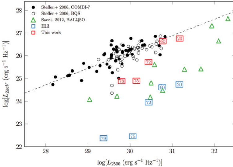
Fig. 5.9 X-ray (2 keV) luminosity of the clumped model ( red squares ) and the H13 model ( blue squares ), plotted against monochromatic luminosity at 2500 Å. The points are labeled according to inclination; angles >70^\circ correspond to BALs in this scheme (see Fig. 5.7). Also plotted are measurements from the COMBI-7 AGN and the BQS samples (Steffen et al. 2006) and the Saez et al. (2012) sample of BALQSOs. The dotted line shows the best fit relation for non-BALQSOs from Steffen et al. (2006)
