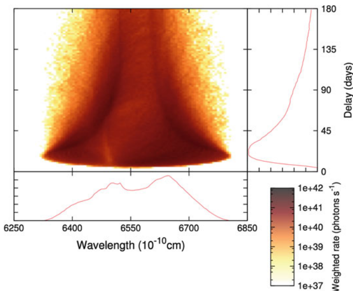
Fig. 7.2 Velocity-resolved transfer function for H\alpha from the fiducial quasar model presented in Chap. 5. The transfer function is for a viewing angle of 40^\circ . Credit Sam Mangham
