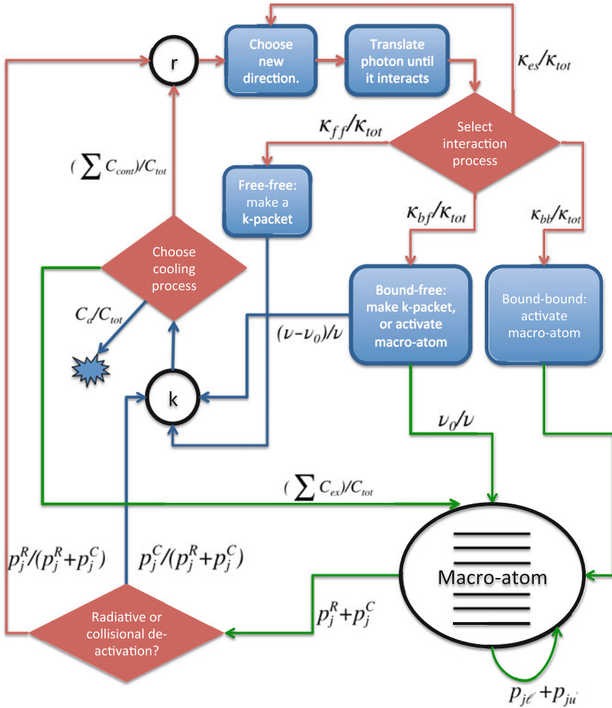
Fig. 3.4 The decision tree traversed by an energy packet in macro-atom mode, depicting the interaction between radiation ( r -packets), the thermal pool ( k -packets), and ionization and ionization/excitation energy (macro-atoms). The probabilities at each decision point are marked, and are defined in the text. The red , blue and green coloured arrows represent radiant, kinetic and ionization/excitation energy respectively. The symbols are defined in the text, except C_{cont} and C_{ex} which refer to cooling contributions to radiative and excitation energy respectively
