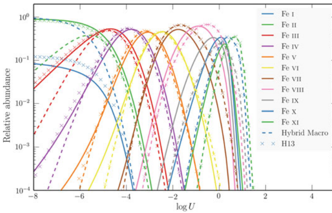
Fig. 3.14 As Fig. 3.9, but for the first 11 ionization stages of iron
