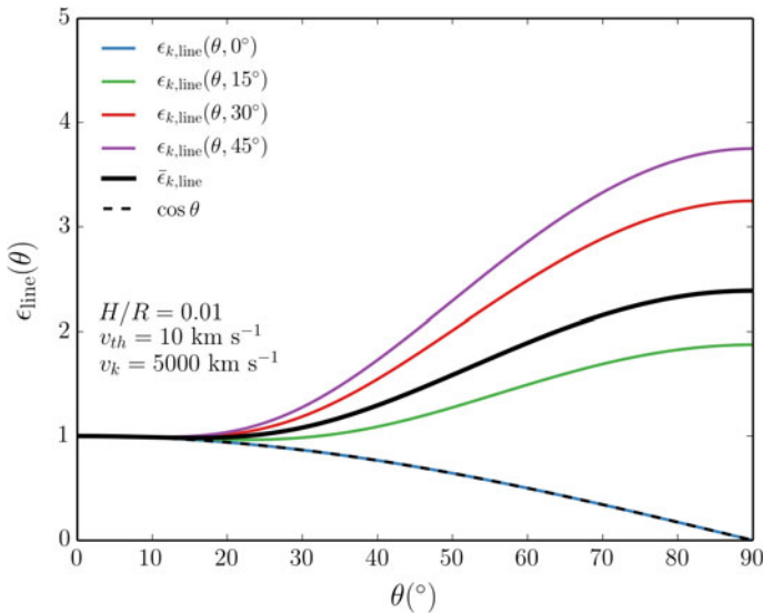
Fig. 6.14 The line angular emissivity function from a Keplerian disc as a function of inclination angle, \theta , for a few different azimuthal angles, \phi . The azimuthally-averaged case, \bar{\epsilon}_{k,\text{line}} (thick black line), and the zero Keplerian velocity shear case, \epsilon_{0,\text{line}}(\theta) = \cos \theta (dotted line), are also shown
