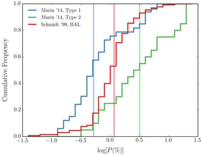
Fig. 6.13 Cumulative distribution functions of the histograms shown in Fig. 6.12 for BAL quasars from Schmidt and Hines (1999) together with the Marin (2014) AGN sample. The colour-coding and x-axis scale are the same as Fig. 6.12. The translucent vertical lines mark the median value in each sample
