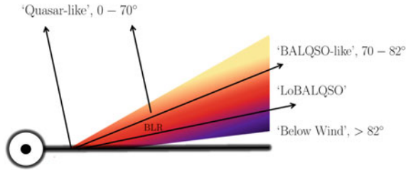
Fig. 5.7 A cartoon describing the broad classes of sightline in the fiducial model, illustrating how geometric effects lead to the different emergent spectra. The colour gradient is approximate, but indicates the stratified ionization structure, from highly ionized ( yellow ) to low ionization ( purple ) material
