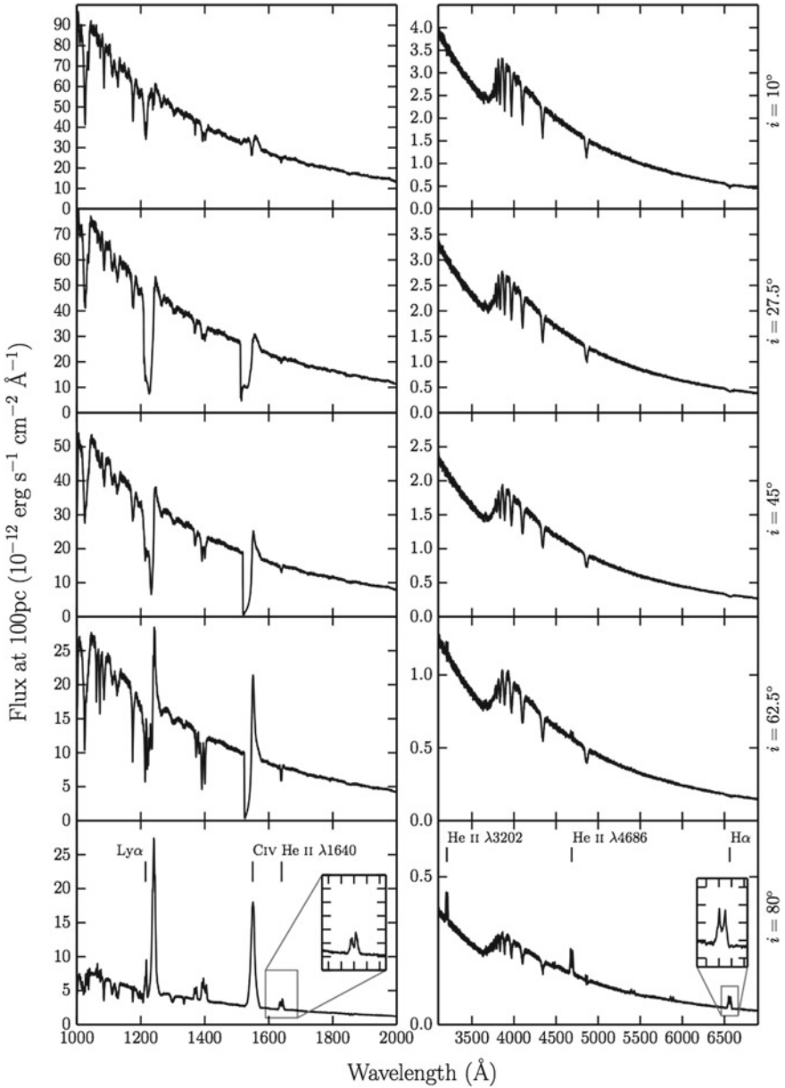
Fig. 4.4 UV ( left ) and optical ( right ) synthetic spectra for model A, the benchmark model, computed at sightlines of 10, 27.5, 45, 62.5 and 80°. The inset plots show zoomed-in line profiles for He II 1640 Å and H \alpha . Double-peaked line emission can be seen in He II 1640 Å, He II 4686 Å, H \alpha and some He I lines, but the line emission is not always sufficient to overcome the absorption cores from the stellar atmosphere models. The model also produces a prominent He II 3202 Å line at high inclinations
