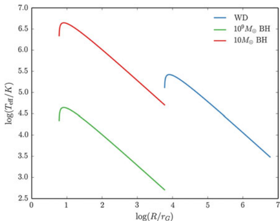
Fig. 1.1 The temperature profile of an accretion disc for three different classes of compact object
