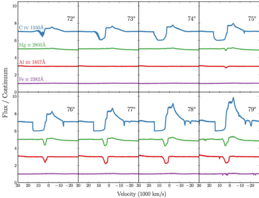
Fig. 5.10 C IV, Mg II, Al III and Fe II line profiles for viewing angles from 72 to 79°. The profiles are plotted relative to the local continuum with an offset applied for clarity. Lower ionization profiles appear at a subset of high inclinations, compared to the ubiquitous C IV profile
