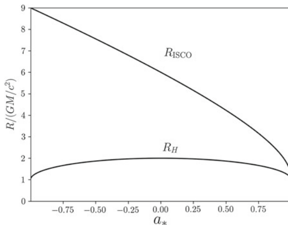
Fig. 1.3 The radius of the ISCO, R_{ISCO} , and the horizon, R_H , is as a function of the BH spin parameter, a_* . a_* = 0 corresponds to a Schwarzschild BH, and a_* = 1 and a_* = -1 to prograde and retrograde Kerr BHs, respectively. Note that this figure ignores the counteracting torque of photons swallowed by the BH, which actually limits a_* to a value of around 0.998 (Thorne 1974)
