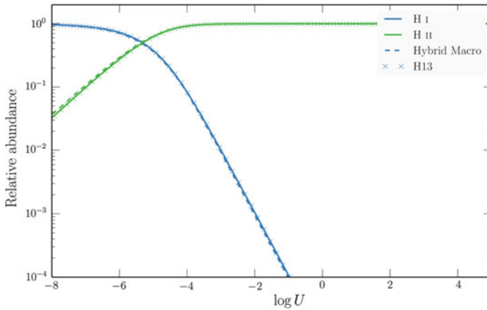
Fig. 3.9 Relative ion fractions as a function of ionization parameter from the hybrid macro-atom scheme, with Hydrogen and Helium treated as a full macro-atom ( dotted lines ), compared to both CLOUDY ( solid lines ) and PYTHON in simple-atom only mode (H13, crosses). The colours correspond to the different ionic stages and are labeled for the CLOUDY case
