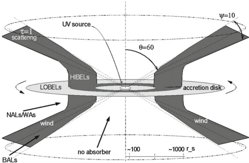
Fig. 2.12 A schematic showing the main features of the Elvis model. A biconical wind rises from an accretion disc, and the observed spectrum is determined purely by the viewing angle of the observer. Credit Martin Elvis
