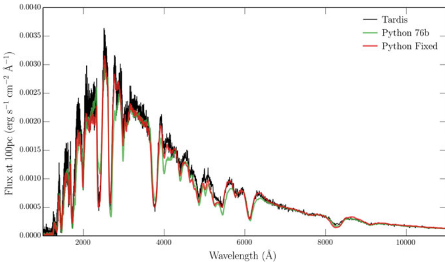
Fig. 3.16 Comparison between TARDIS and PYTHON synthetic spectra from a simple 1D supernova model. A bug in Doppler shifting of photons was discovered around PYTHON 76, meaning that the code now gives even better agreement than presented in Kerzendorf and Sim (2014)
