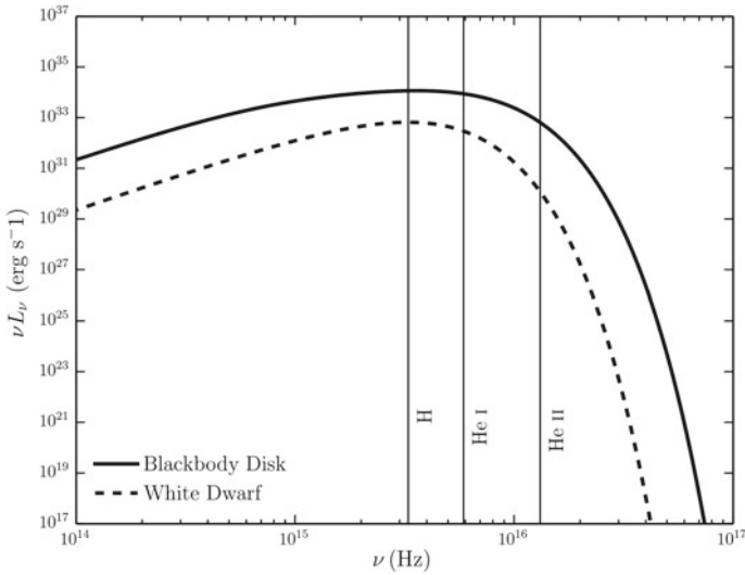
Fig. 4.2 The spectral energy distribution of the accretion disc and white dwarf used in the ionization cycles for the CV modelling. The important ionization edges for hydrogen and helium are marked
