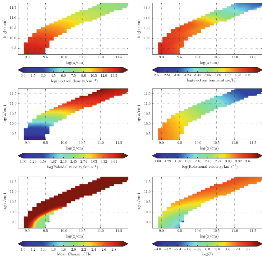
Fig. 4.3 The physical properties of the wind—note the logarithmic scale. Near the disc plane the wind is dense, with low poloidal velocities. As the wind accelerates it becomes less dense and more highly ionized. The dominant He ion is almost always He III, apart from in a small portion of the wind at the base, which is partially shielded from the inner disc
