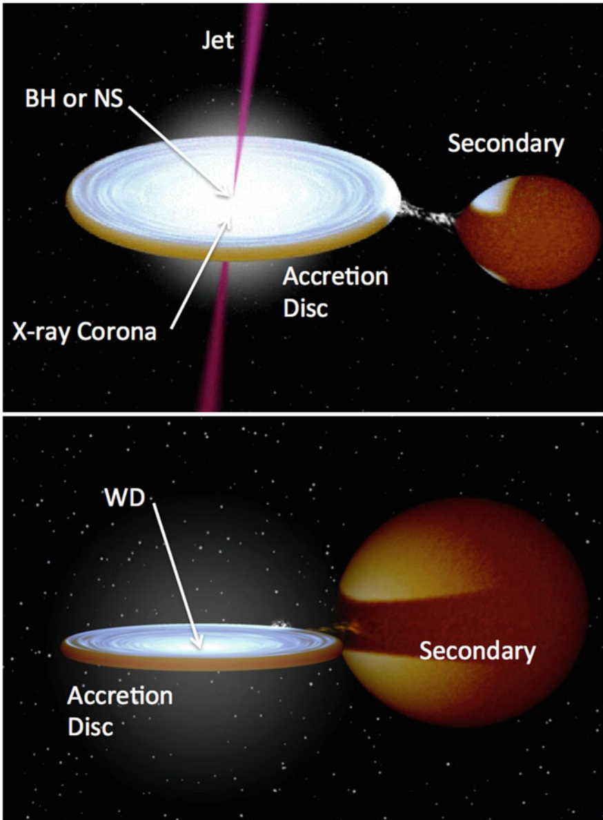
Fig. 1.6 Artist's impression of a low-mass X-ray binary ( top ) and cataclysmic variable ( bottom ). The key components are marked, and the clear similarity in overall structure is apparent. Credit Rob Hynes
