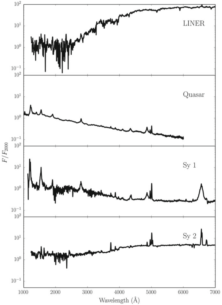
Fig. 1.12 Template spectra, from the AGN atlas, for four common types of AGN. Obtained from http://www.stsci.edu/hst/observatory/crds/cdbs_agn.html
