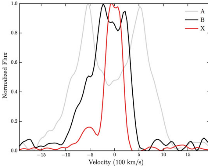
Fig. 4.10 H\alpha line profiles, normalized to 1, plotted in velocity space for three models with varying kinematic properties, computed at an inclination of 80^\circ . The benchmark model and the improved optical model described in Sect. 4.3 are labeled as A and B respectively, and a third model (X) which has an increased acceleration length of R_v = 283.8 R_{WD} , and \alpha = 4 is also shown. The x -axis limits correspond to the Keplerian velocity at 4 R_{WD} , the inner edge of the wind. There is a narrowing of the lines, and a single-peaked line in model X. This is not due to radial velocity shear (see Sect. 4.3.3)
