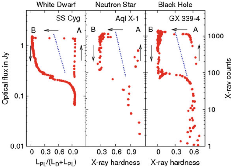
Fig. 1.16 Hardness-intensity diagrams for three types of accreting compact objects: the dwarf nova SS Cyg ( left ), in addition to neutron star ( middle ) and black hole ( right ) LMXBs. The dotted line shows the ‘jet line’ in LMXBs and the arrows show the expected temporal evolution of the system. For SS Cyg the x -axis shows the fraction of the hard X-ray power law component in the system compared to the luminosity of the combined luminosity of disc and power law. This quantity is analogous to the X-ray hardness in LMXBs. Credit Fig. 1.1. K rding et al. 2008, Science, 320, 1318. Reprinted with permission from AAAS
