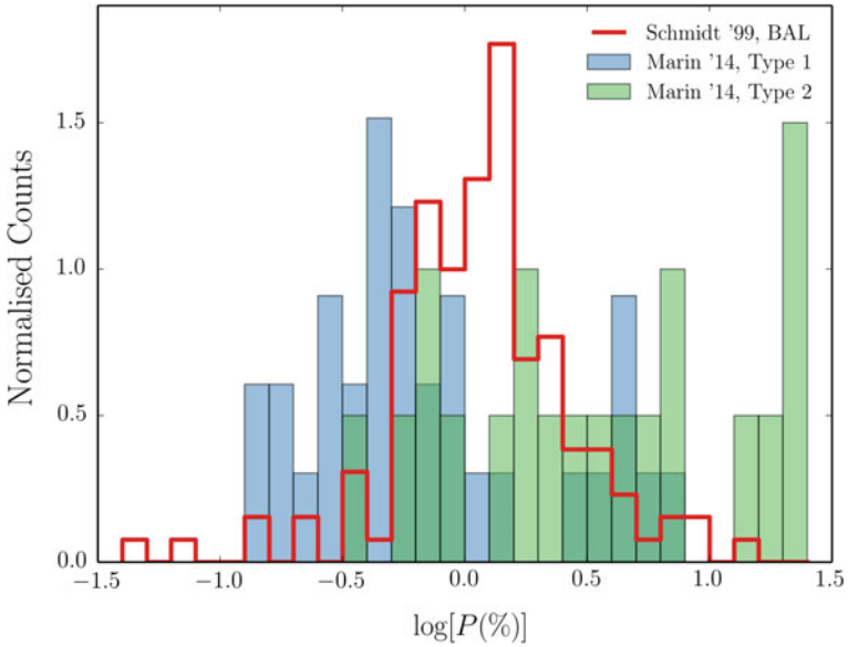
Fig. 6.12 Histograms of polarisation percentages for BAL quasars from Schmidt and Hines (1999) together with the Marin (2014) AGN sample
