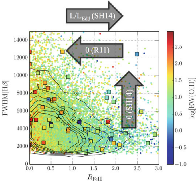
Fig. 6.10 Eigenvector 1 for LoBAL and non-BAL quasars. FWHM of the H \beta line plotted against the relative iron strength, R_{\text{FeII}} . The colour coding corresponds to the EW of [O III] 5007 Å. The dots mark all quasars from sample A, while the squares mark those with Mg II LoBALs. A few of the Mg II LoBALQSOs are missing due to their lack of FWHM[H \beta ] measurements. The arrows show the approximate direction of the expected inclination ( \theta ) trend under both the SH14 and R11 interpretations, and the expected trend in Eddington fraction ( L/L_{\text{Edd}} ) from SH14 only
