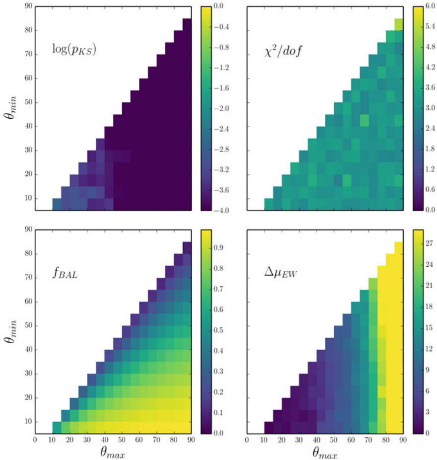
Fig. 6.9 Heat map showing the results of the MC simulation described in Sect. 6.4.2, but this time conducted with a Log-normal intrinsic distribution. The quantities shown are the same as in Fig. 6.8. Note the different scale for the colour coding of the \chi^2/dof panel ( upper right )
