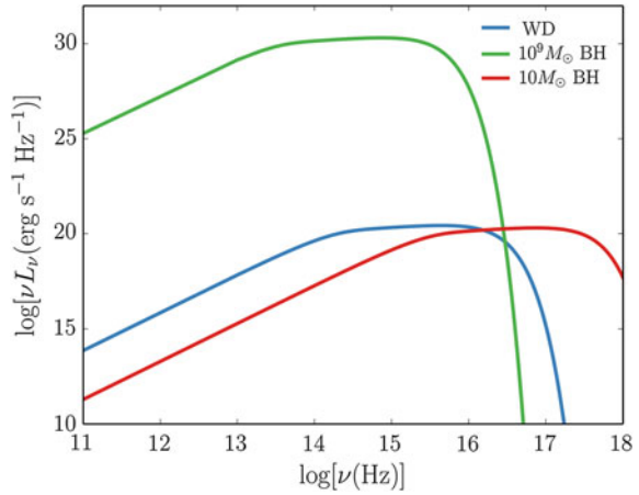
Fig. 1.4 Accretion disc SEDs for three different compact objects, corresponding roughly to a quasar, an XRB and a CV. The SEDs are computed via an area-weighted sum of blackbodies with effective temperatures governed by Eq. 1.19, and the \nu^{1/3} shape in the middle of the spectra can be seen
