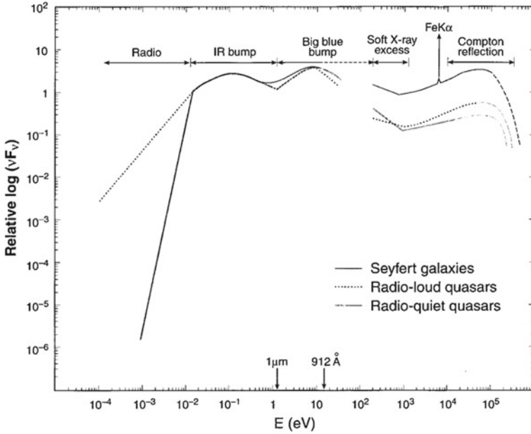
Fig. 1.14 Approximate average broadband SEDs for a few types of AGN. The series of characteristic bumps can be clearly seen. The Soft-X-ray excess is also visible (see Sect. 1.3.2.1). Credit Koratkar and Blaes (1999). Copyright PASP, reprinted by permission of the authors.
