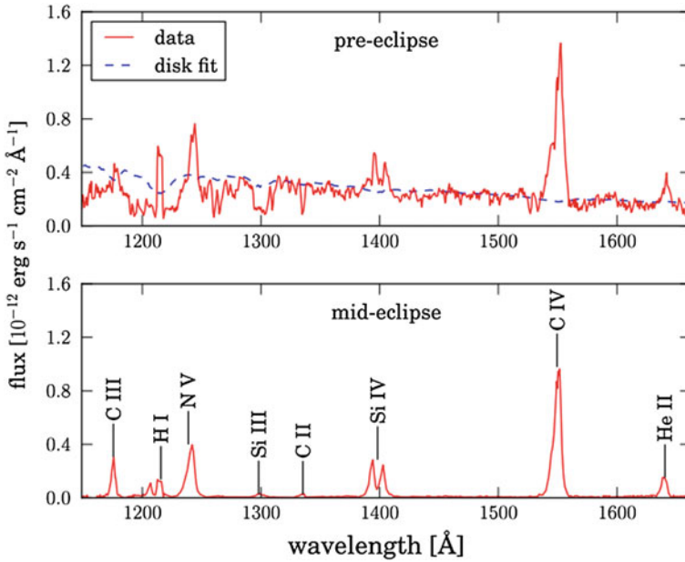
Fig. 1.10 UV spectrum of RW Tri in and out of eclipse, showing strong lines in C IV 1550 Å and Ly \alpha , among others. Credit Noebauer et al. 2010. Copyright AAS. Reproduced with permission
