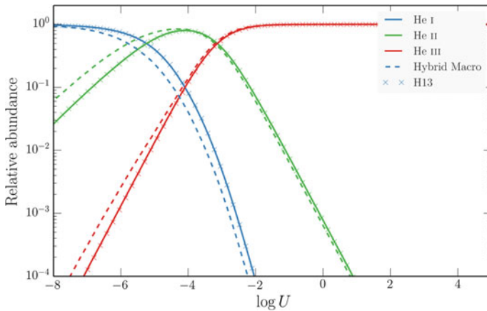
Fig. 3.10 As Fig. 3.9, but for Helium
